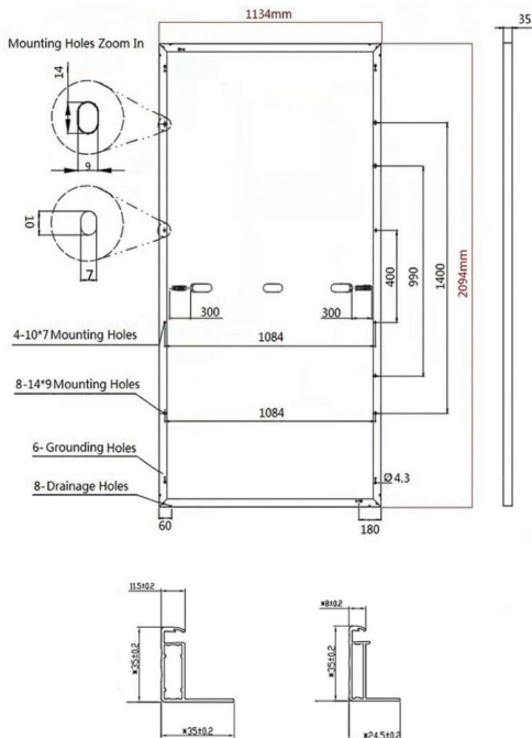
Dimensions of PV Module Unit: mm
